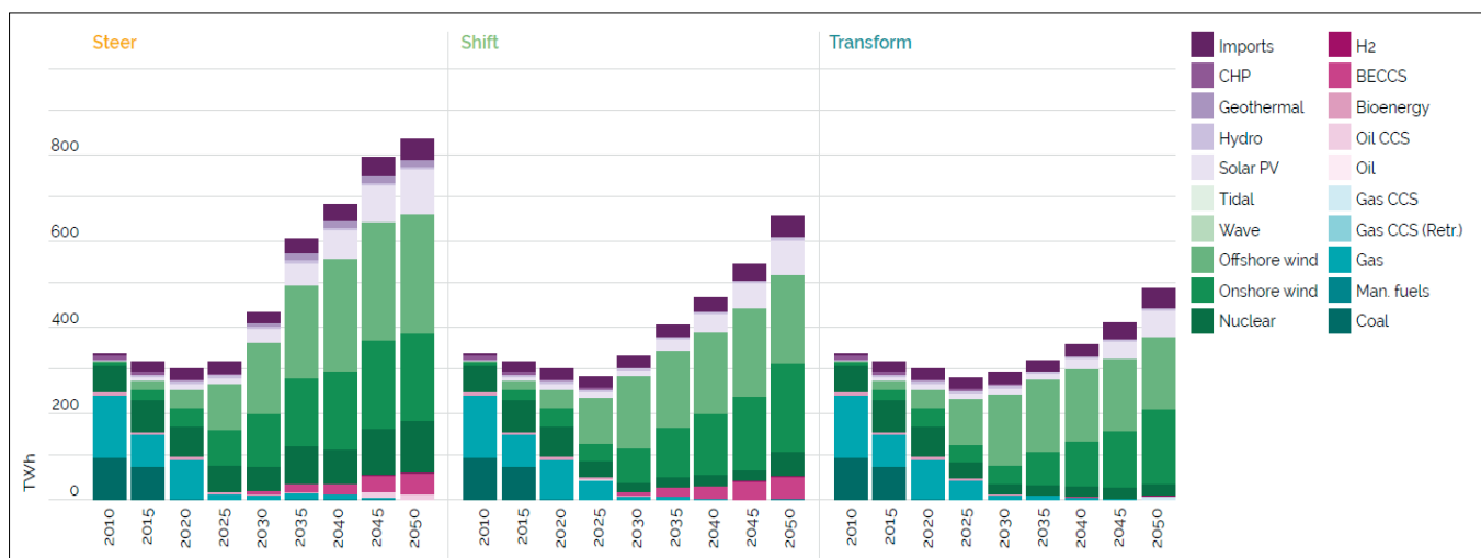
Figure 1: Power generation by scenario 'Steer', 'Shift' or 'Transform', 2010–2050.
