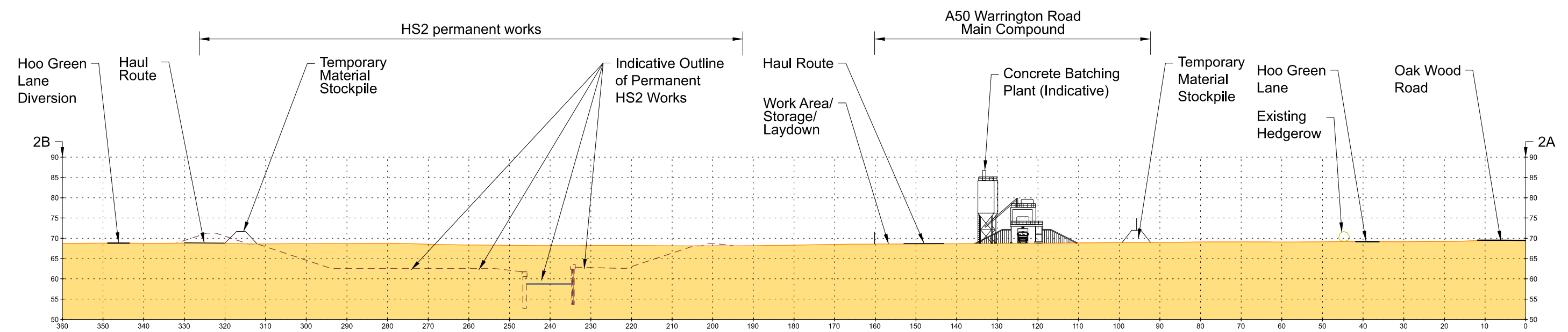
INDICATIVE SECTION 2A-2B SCALE 1:1000 For Plan refer to 2PT24-MWJ-PT-MAP-M000-002232-HS2-022
