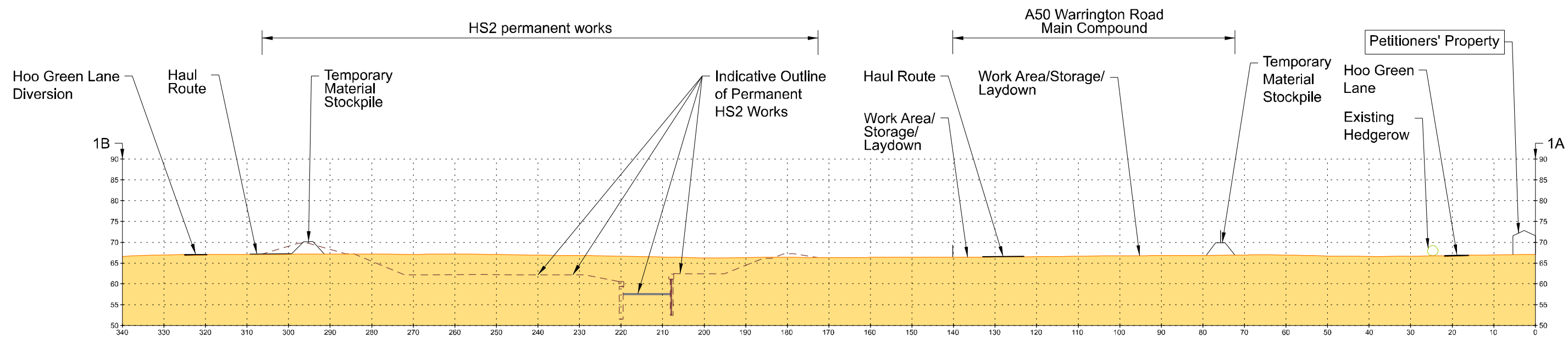
INDICATIVE SECTION 1A-1B SCALE 1:1000 For Plan refer to 2PT24-MWJ-PT-MAP-M000-002232-HS2-022
