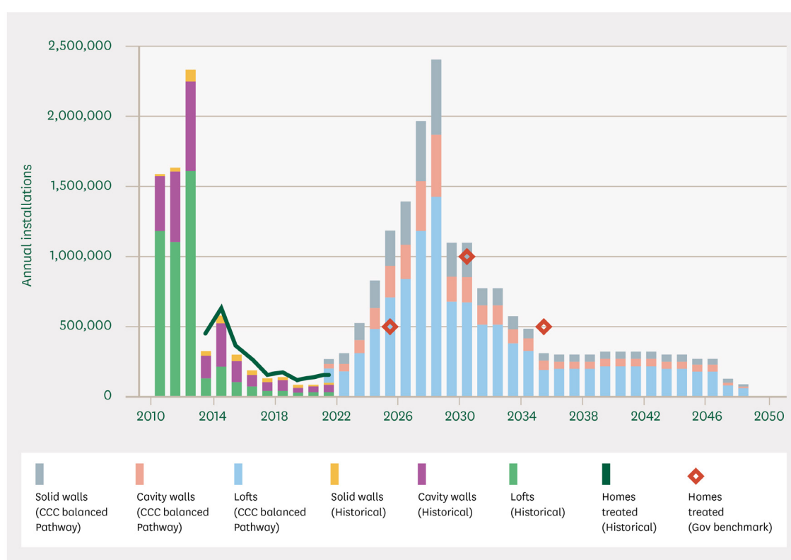
Figure 2: Energy efficiency installations 2010–2022 and projected pathway
